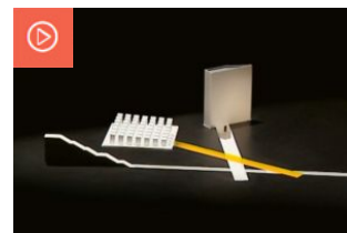
Architectures
